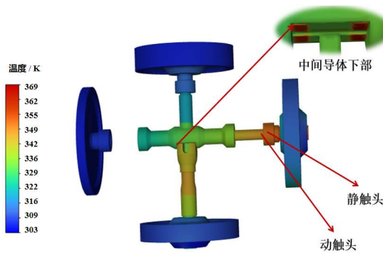
图 5 GIS 三工位温度仿真结果图 Fig. 5 GIS three-position temperature simulation results
