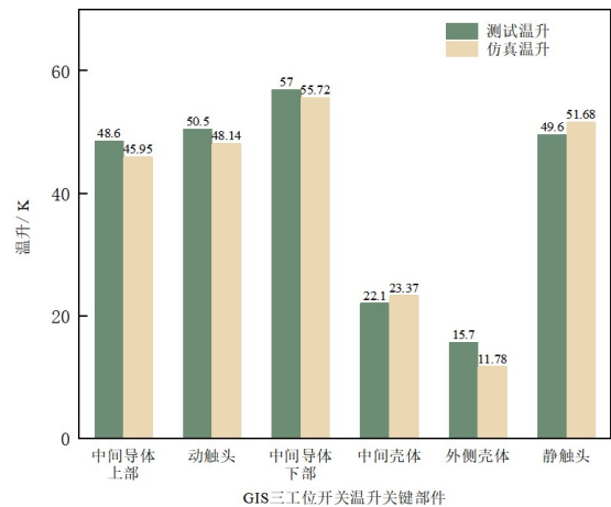
图 8 温升测试和仿真结果对比图 Fig. 8 CoMParison of temperature rise test and simulation results
