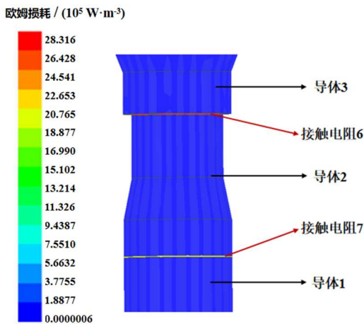
图 3 导体连接处的功率密度 Fig. 3 Power density at the conductor joint
