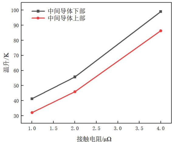
图 10 中间导体上下部分随接触电阻 5 的温升变化情况 Fig. 10 Temperature rise of the upper and lower part of the intermediate conductor with contact resistance 5
