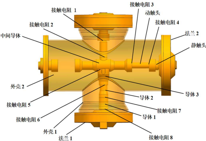
图 1 简化模型整体图 Fig. 1 Simplified model overall diagram
