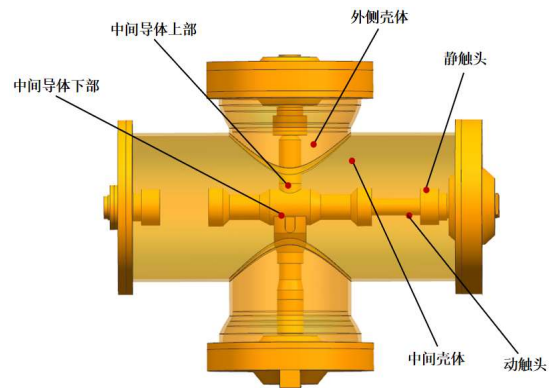
图 7 GIS 三工位开关温升实验测温点 Fig. 7 Temperature rise test measurement points for GIS three-position switch
